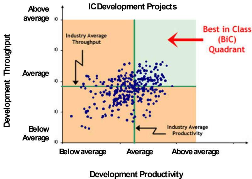
Figure 1: Identifying Best-in-class
